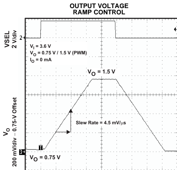
t – Time = 50 \mu s/div
