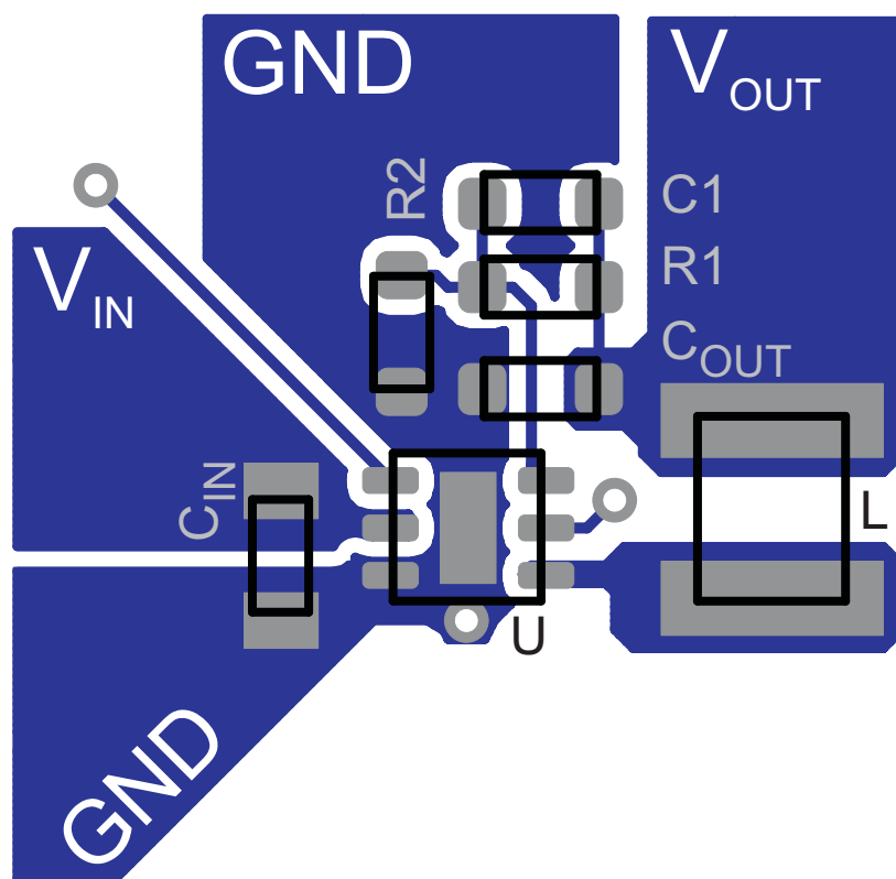
Figure 24. Layout Recommendation
