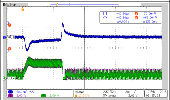
Figure 30. Load Transient Response (PWM-PWM)
