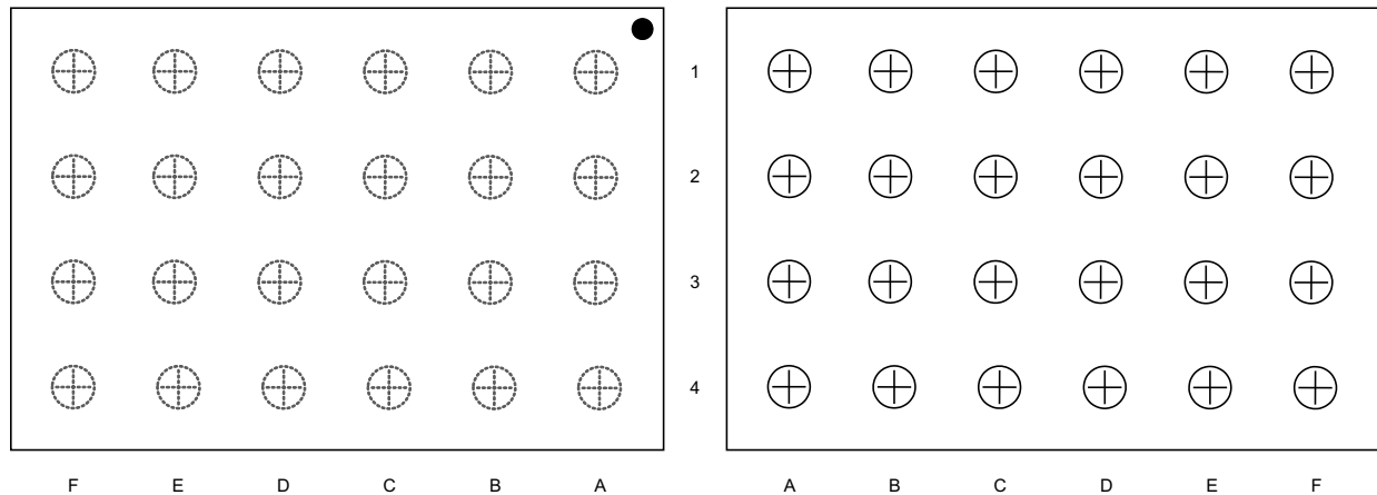
Pin Functions
