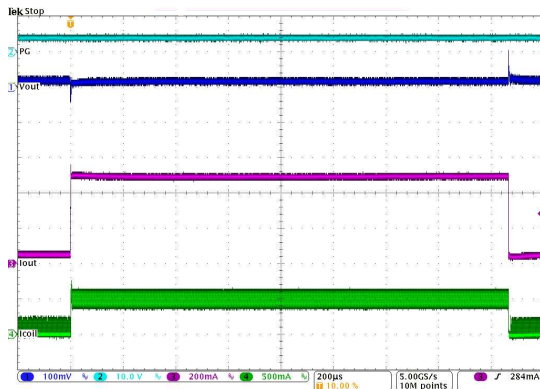
Figure 35. Load Transient Response, Power Save Mode, I_{OUT} (50 mA to 500 mA)
