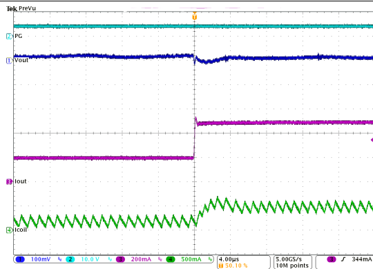
Figure 33. Load Transient Response, PWM Mode, I_{OUT} (200 mA to 500 mA), Rising Edge
