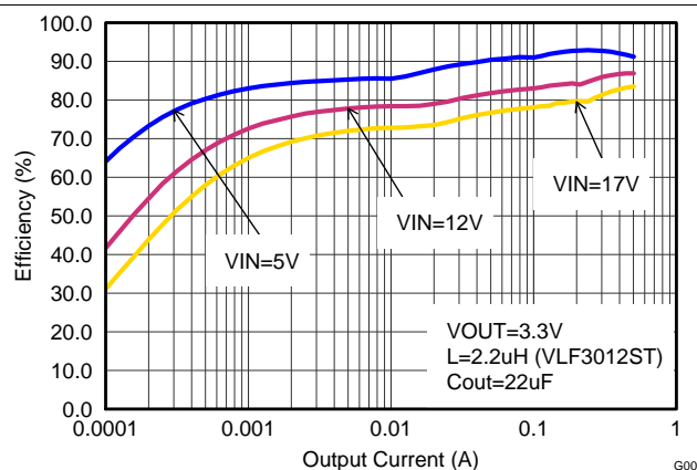
Figure 12. Efficiency vs Output Current, V_{OUT} = 3.3 V
