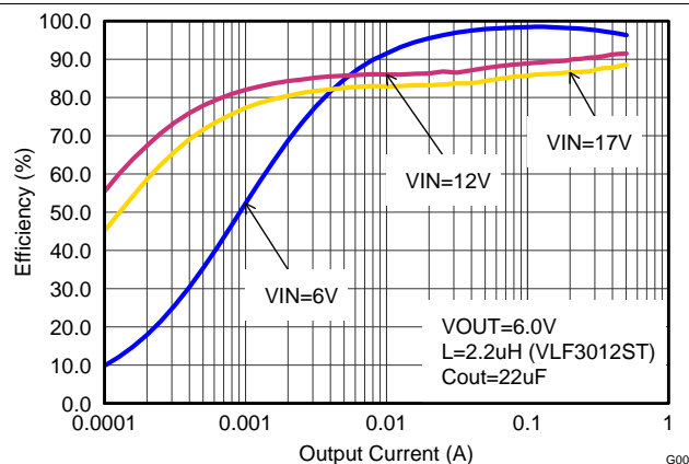
Figure 8. Efficiency vs Output Current, V_{OUT} = 6 V
