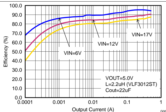
Figure 10. Efficiency vs Output Current, V_{OUT} = 5 V
