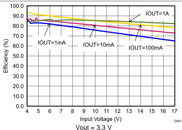
Figure 11. Efficiency versus Input Voltage
