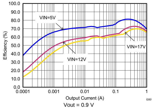
Figure 14. Efficiency versus Output Current
