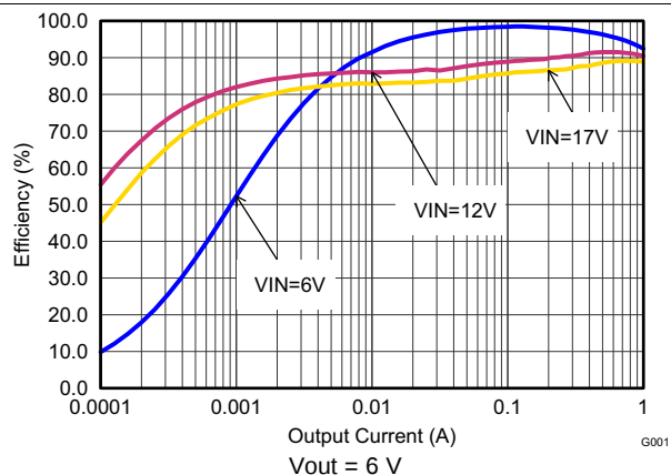
Figure 8. Efficiency versus Output Current
