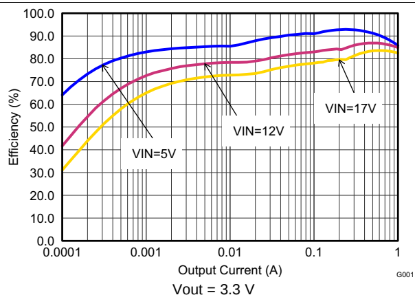
Figure 10. Efficiency versus Output Current
