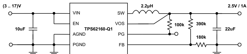
Figure 35. 2.5-V/1-A Power Supply
