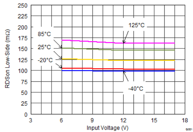
Figure 4. Low-Side Static Drain-Source-Resistance ( R_{DS(on)} )
