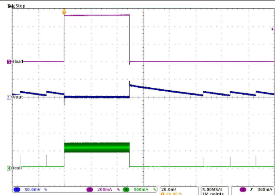
Figure 23. PWM to PSM Mode Transition
