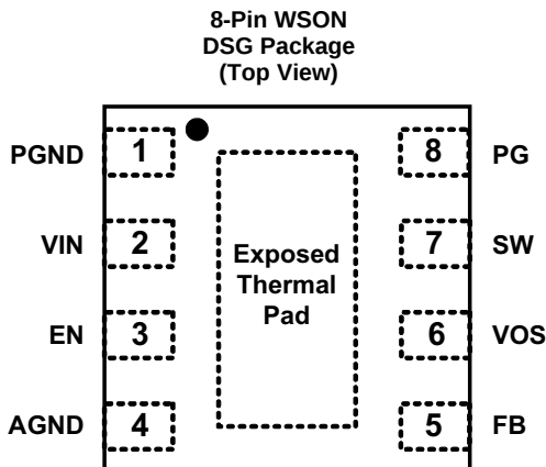
Pin Functions
