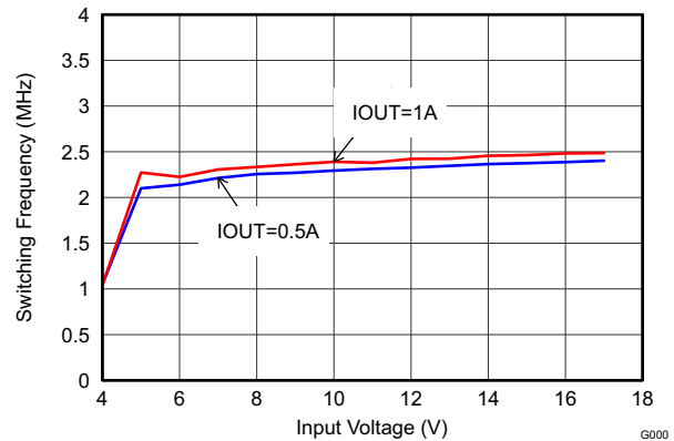
Figure 19. Switching Frequency versus Input Voltage
