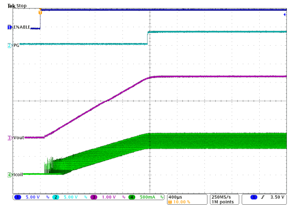
Figure 9-35. Start-Up Into 1 A
