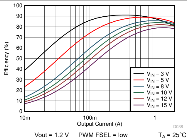
Figure 10-5. Efficiency vs Output Current
