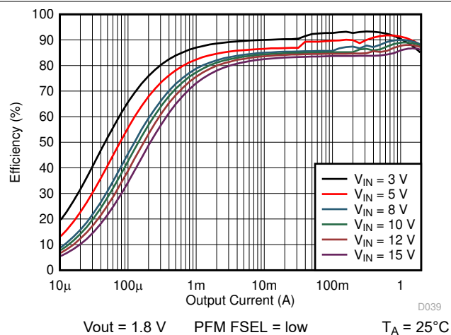
Figure 10-7. Efficiency vs Output Current
