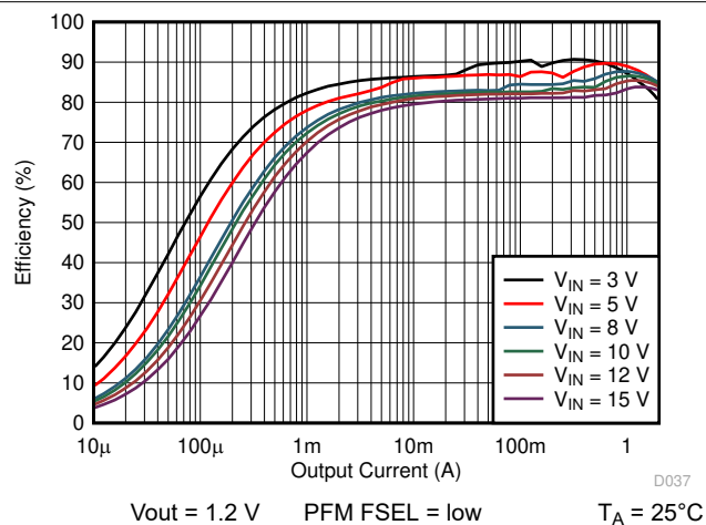
Figure 10-3. Efficiency vs Output Current
