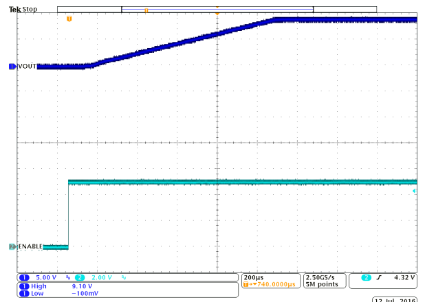
Figure 10-63. Start-Up Timing
