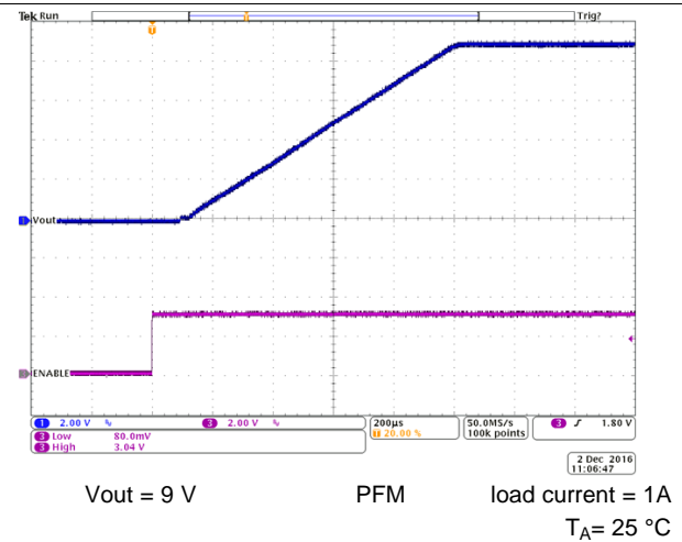
Figure 63. Start-Up Timing
