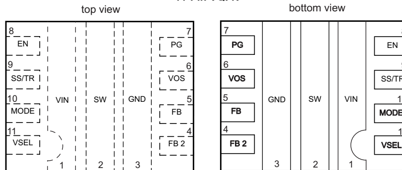
RGX Package 11-Pin VQFN
