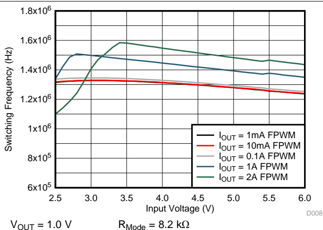
Figure 15. Switching Frequency, Forced PWM Mode (1.5 MHz)
