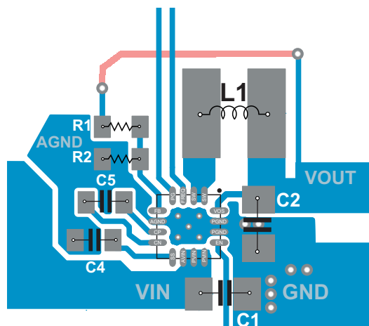
Figure 29. TPS6209x Layout
