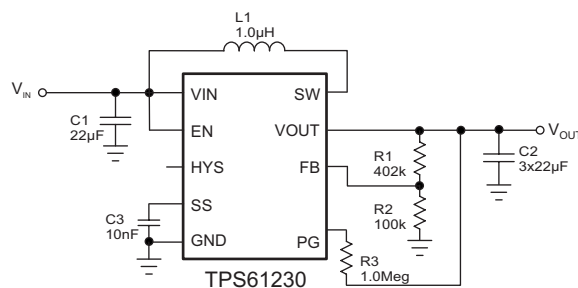
Figure 12. TPS61230 5-V Output Typical Application
