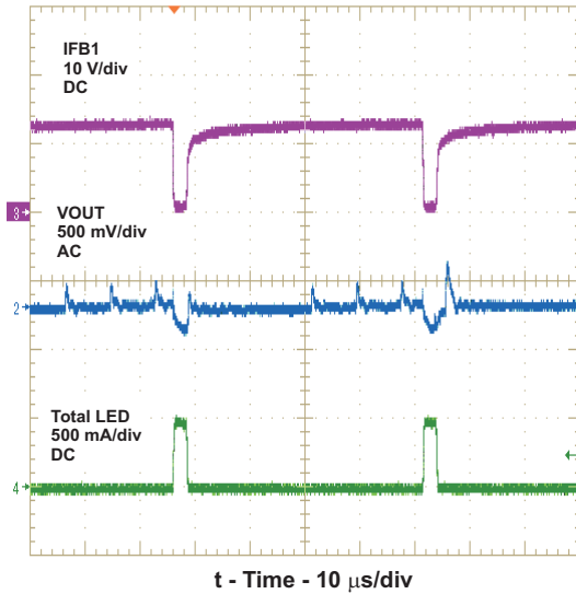
Figure 5. Dimming Waveforms
