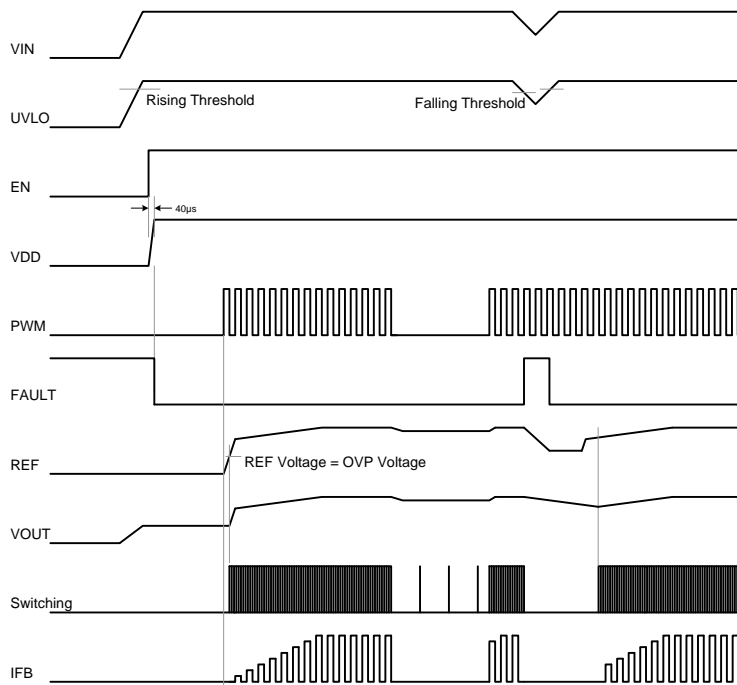
Figure 16. Power-Up Sequencing
