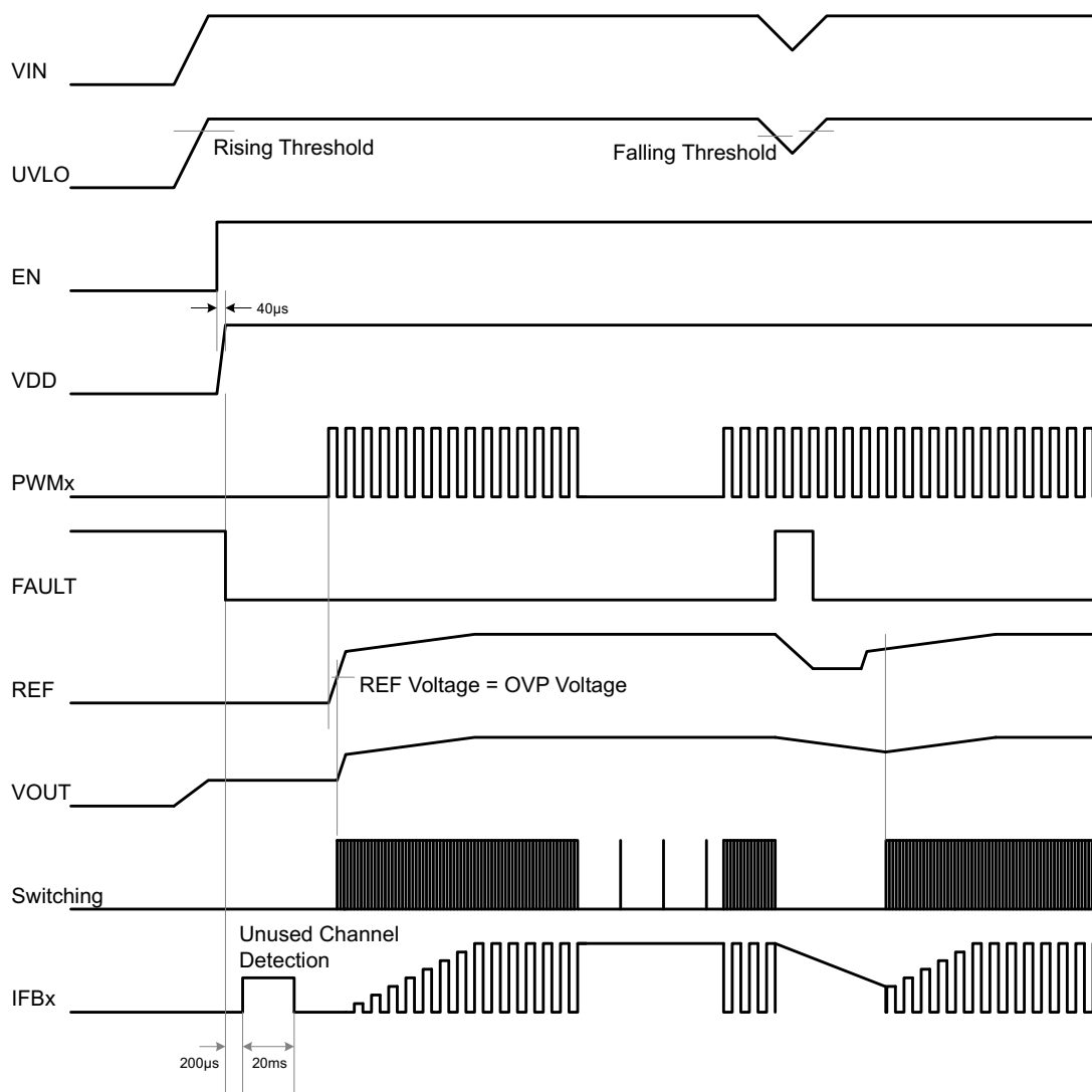
Figure 20. Power-Up Sequencing
