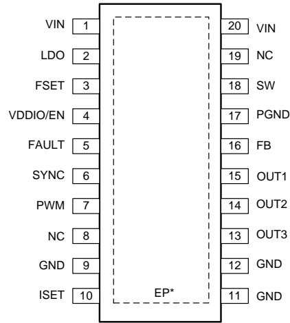
PWP Package 20-Pin TSSOP With Exposed Thermal Pad Top View
