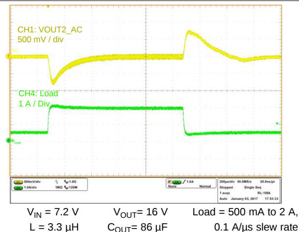
Figure 30. Load Transient
