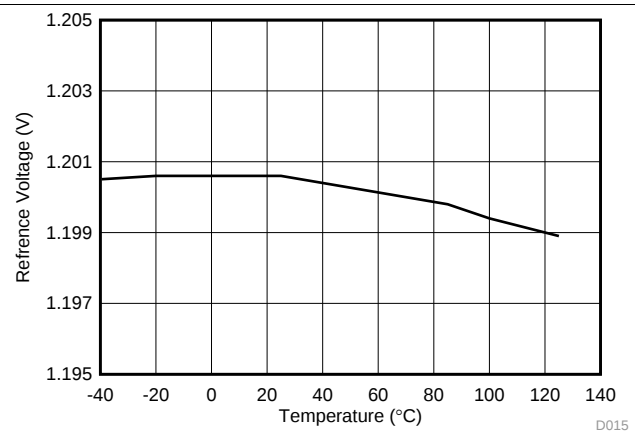
Figure 14. Reference Voltage vs Temperature
