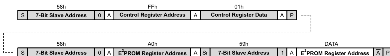
Figure 33. Reading From A Single E 2 PROM Register
