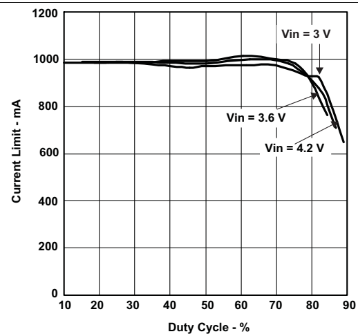
Figure 2. Overcurrent Limit (Dual Output) vs Duty Cycle
