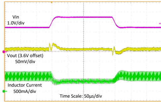
Figure 8-9. Line Transient
