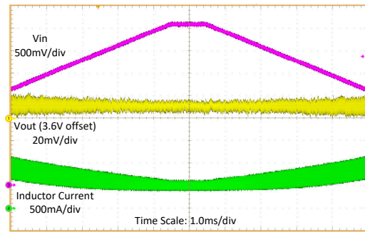
Figure 8-9. Line Transient
