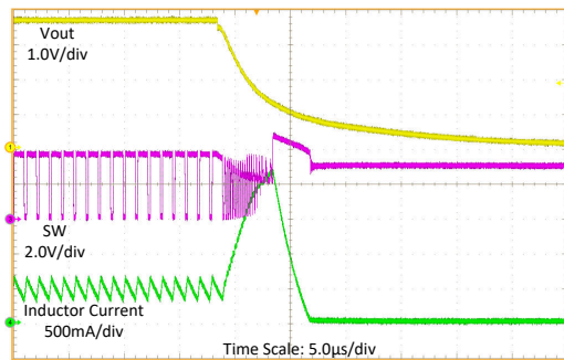
Figure 8-10. Load Sweep
