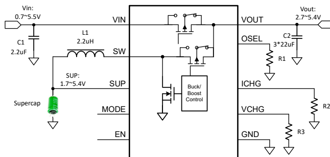
Typical Application Circuit 1
