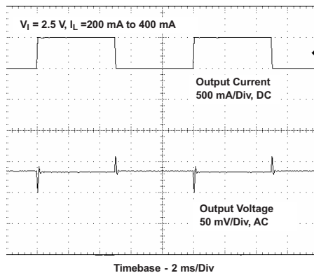
Figure 17. Load Transient Response
