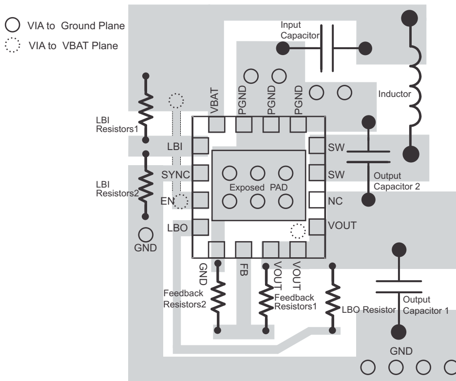
Figure 23. Layout Example Schematic
