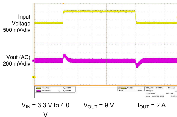
Figure 9-8. Line Transient
