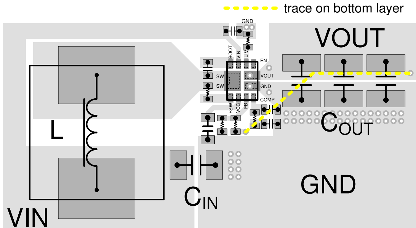
Figure 11-1. Layout Example
