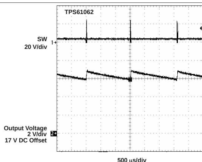
Figure 15. Overvoltage Protection
