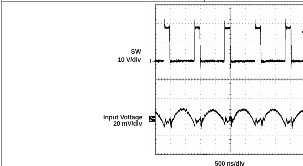
Figure 16. Input Voltage Ripple
