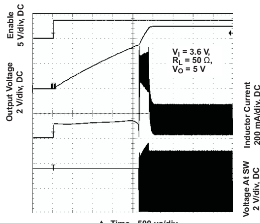
Figure 25. TPS61027 Start-Up After Enable
