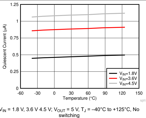
Figure 6-6. Quiescent Current into VIN vs Temperature
