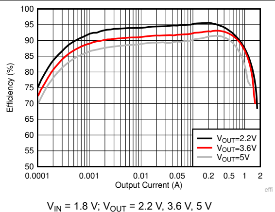
Figure 6-2. Load Efficiency With Different Output
