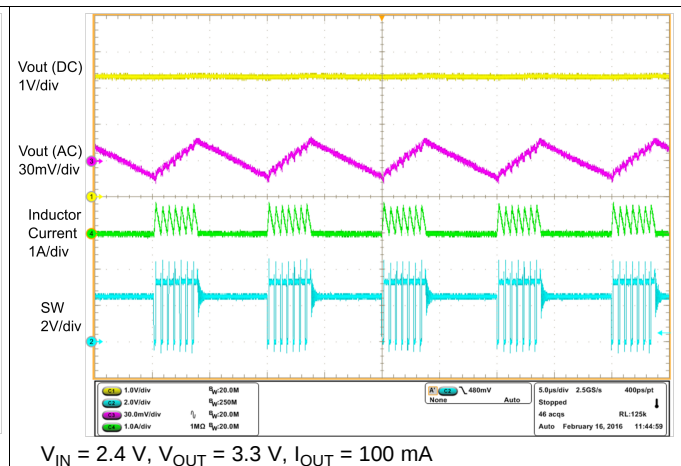
Figure 13. Switching Waveform at Light Load
