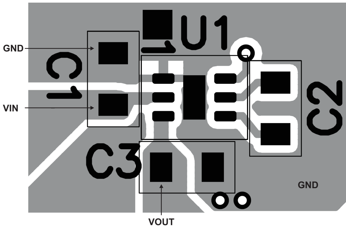
Figure 24. Recommended PCB Layout
