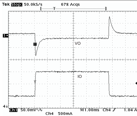
Figure 52. Load Transient
