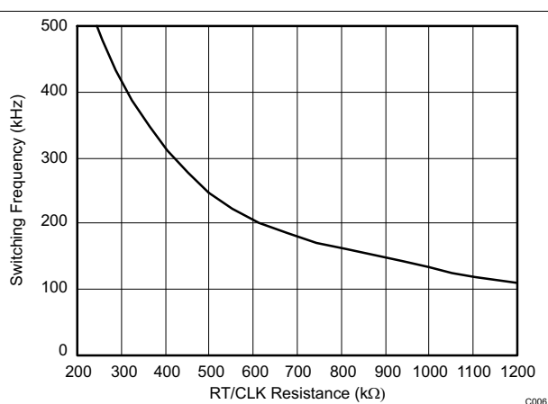
Figure 33. Low-Range RT
