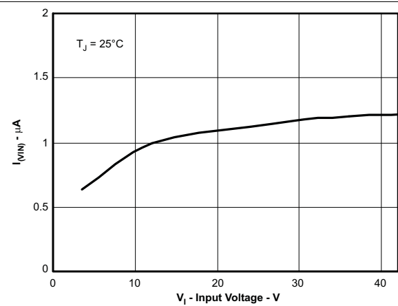
Figure 17. Shutdown Supply Current vs Input Voltage ( V_{IN} )
