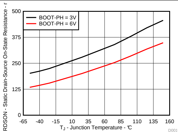
Figure 2. On Resistance vs Junction Temperature
