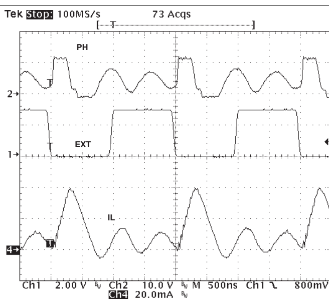
Figure 44. Plot of Synchronizing in DCM
