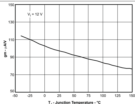
Figure 8. EA Transconductance vs Junction Temperature
