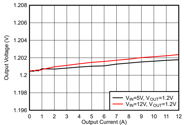
Figure 6-24. Load Regulation, f_{sw} = 800\text{ kHz}
