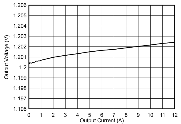
Figure 8-3. Load Regulation
