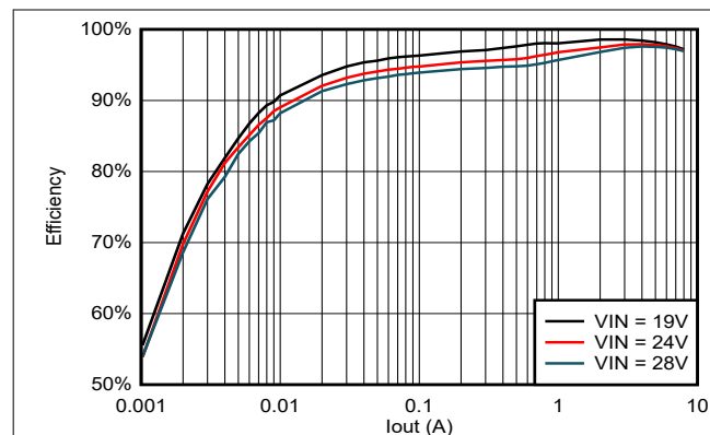
Figure 5-13. Efficiency, Vout = 15V
