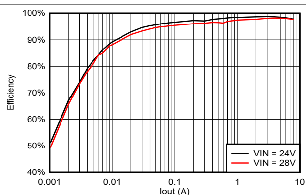
Figure 5-14. Efficiency, Vout = 20V
