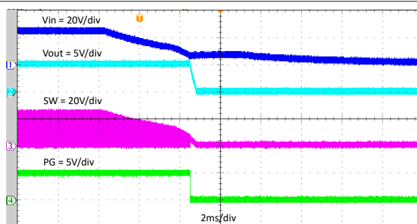
Figure 7-15. Shutdown Relative to V_{IN}
