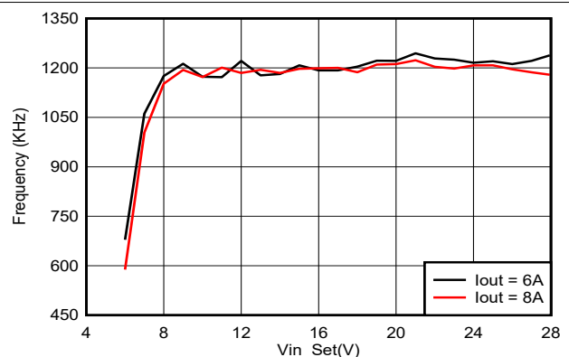
Figure 5-12. Switching Frequency vs Input Voltage, Vout = 5V, Fsw = 1200kHz
