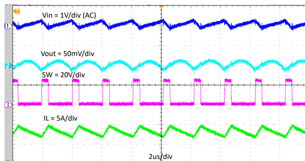
Figure 7-9. Steady State Waveforms, I_{OUT} = 8A
