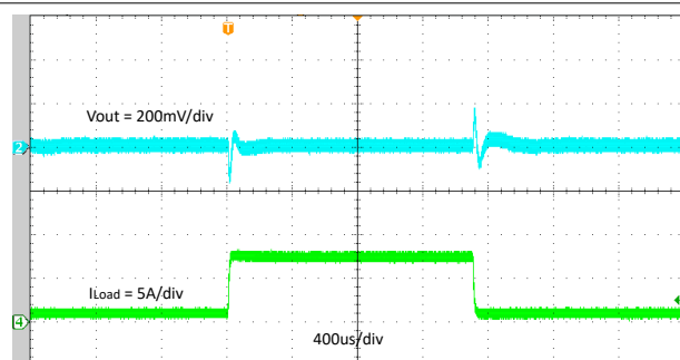
Figure 7-12. Transient Response 0.8A to 7.2A
