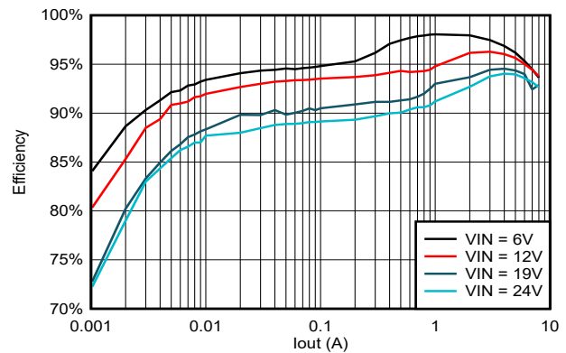
Figure 5-18. TPS56837 Efficiency, V_{out} = 5V , F_{sw} = 800kHz
