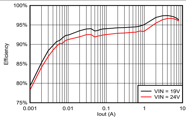
Figure 5-21. TPS56837 Efficiency, V_{out} = 12V , F_{sw} = 800kHz
