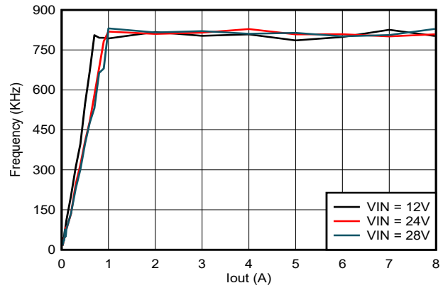
Figure 5-14. TPS56837 Switching Frequency vs Output Current, V_{out} = 5V , F_{sw} = 800kHz
