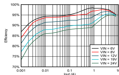
TPS56837 Efficiency, Vout = 5V, Fsw = 500kHz
