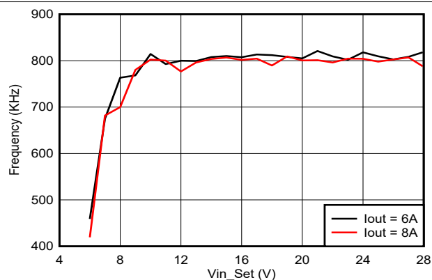
Figure 5-11. Switching Frequency vs Input Voltage, Vout = 5V, Fsw = 800kHz
