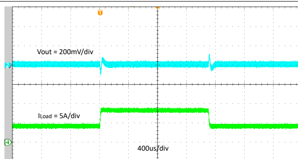
Figure 7-13. Transient Response 4A to 8A
