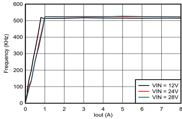
Figure 5-13. TPS56837 Switching Frequency vs Output Current, V_{out} = 5V , F_{sw} = 500kHz
