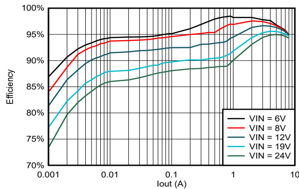
Figure 5-17. TPS56837 Efficiency, V_{out} = 5V , F_{sw} = 500kHz
