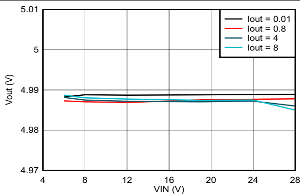
Figure 7-4. Line Regulation
