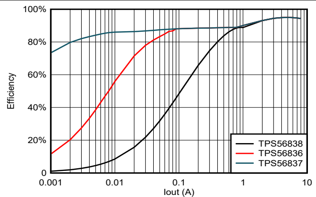
Figure 5-22. TPS56837, TPS56838 and TPS56836 Efficiency, V_{in} = 24V , V_{out} = 5V , F_{sw} = 500kHz
