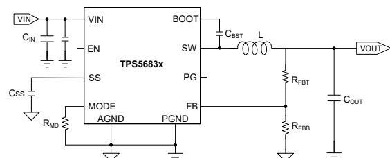
Simplified Schematic
