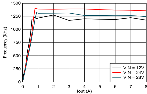
Figure 5-15. TPS56837 Switching Frequency vs Output Current, V_{out} = 5V , F_{sw} = 1200kHz
