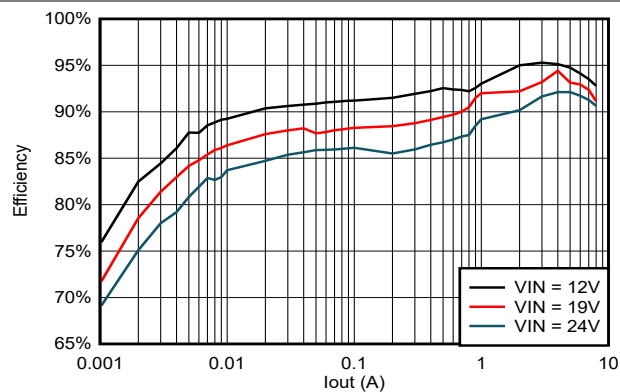
Figure 5-19. TPS56837 Efficiency, V_{out} = 5V , F_{sw} = 1200kHz
