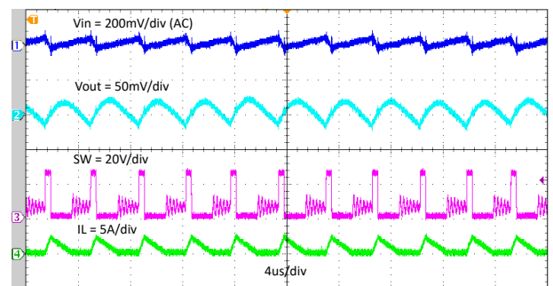
Figure 7-7. Steady State Waveforms, IOUT = 0.6A
