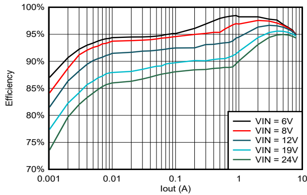
Figure 7-2. Efficiency
