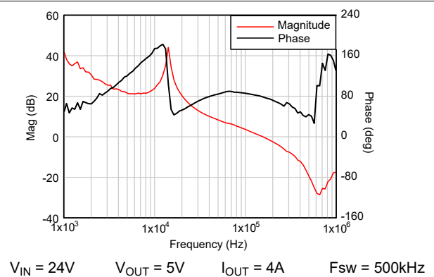
Figure 7-5. Bode Plot
