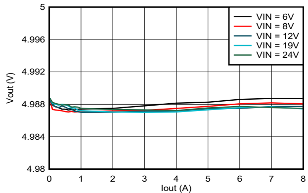
Figure 7-3. Load Regulation
