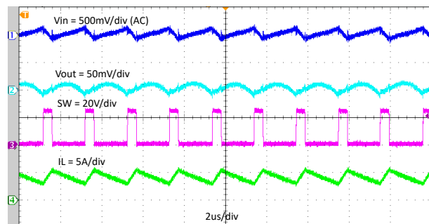
Figure 7-8. Steady State Waveforms, I_{OUT} = 4A
