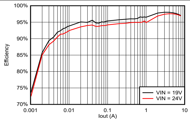
Figure 5-20. TPS56837 Efficiency, V_{out} = 12V , F_{sw} = 500kHz
