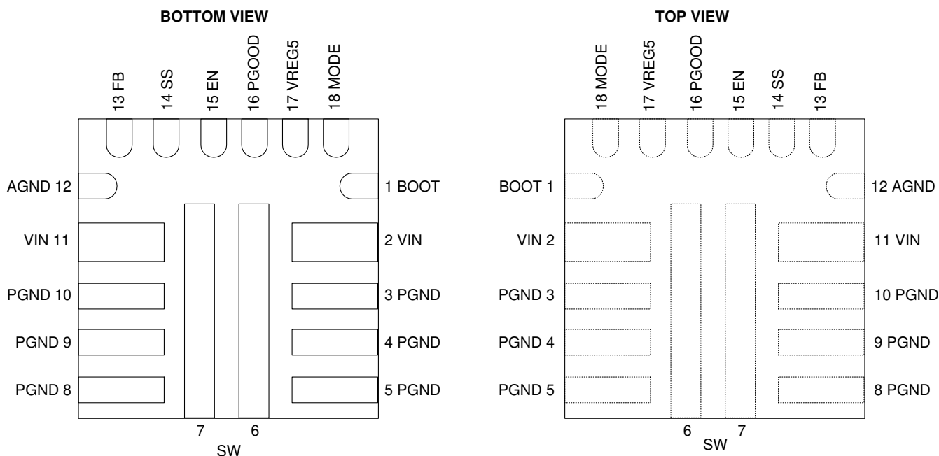
Figure 5-1. 18-Pin VQFN RNN Package (Bottom View Left, Top View Right)
