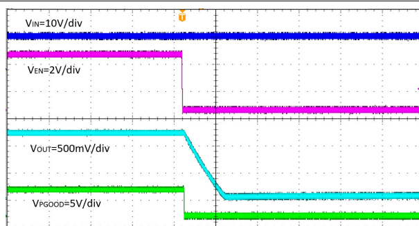
Figure 8-7. Shutdown Relative to EN Falling, Time = 200 \mu\text{s/div}
