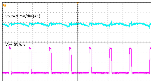
Figure 8-5. Output Voltage Ripple, I_{OUT} = 8\text{ A} , Time = 1 \mu\text{s/div}
