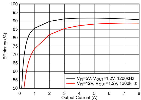
Figure 6-22. Efficiency, Mode = FCCM, f_{sw} = 1200\text{ kHz}
