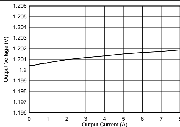
Figure 8-3. Load Regulation
