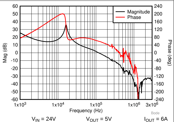
Figure 21. Bode Plot
