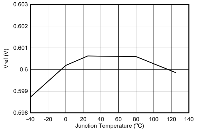
Figure 6-8. V_{REF} Voltage
