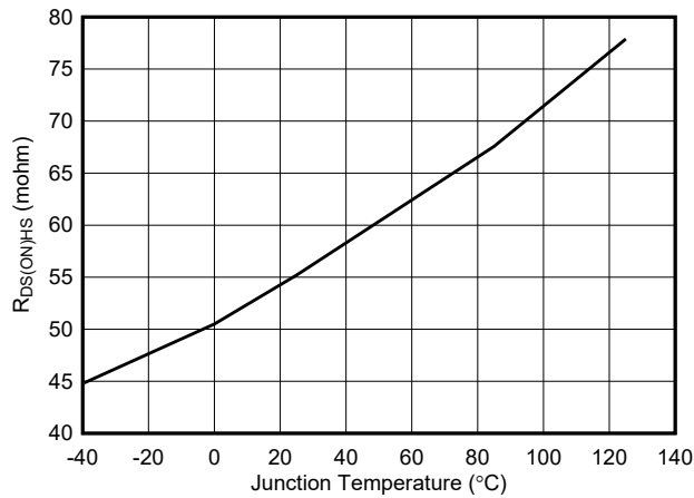
Figure 6-7. High-Side R_{DS(on)}
