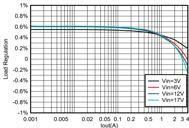
Figure 8-6. TPS564257 Load Regulation vs Loading
