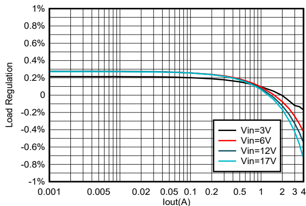
Figure 8-7. TPS564255 Load Regulation vs Loading
