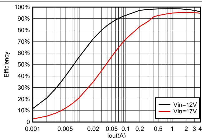
Figure 6-23. TPS564257 Efficiency at 10 V OUT with a 6.8-μH Inductor
