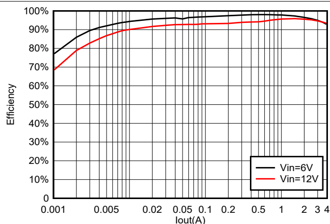
Figure 6-19. TPS564252 Efficiency at 5 V OUT with a 4.7-μH Inductor
