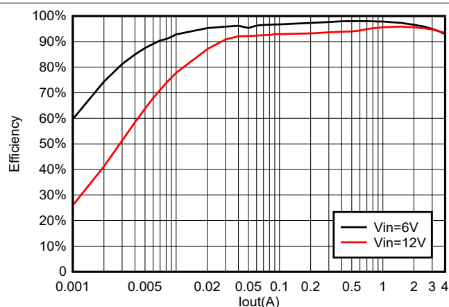
Figure 6-21. TPS564255 Efficiency at 5 V OUT with a 4.7-μH Inductor
