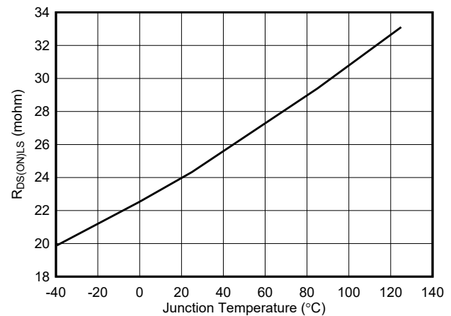
Figure 6-6. Low-Side R_{DS(ON)}
