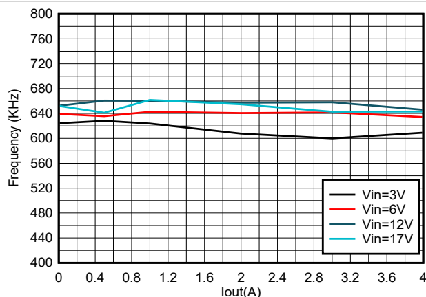
Figure 8-3. TPS564257 Frequency vs Loading
