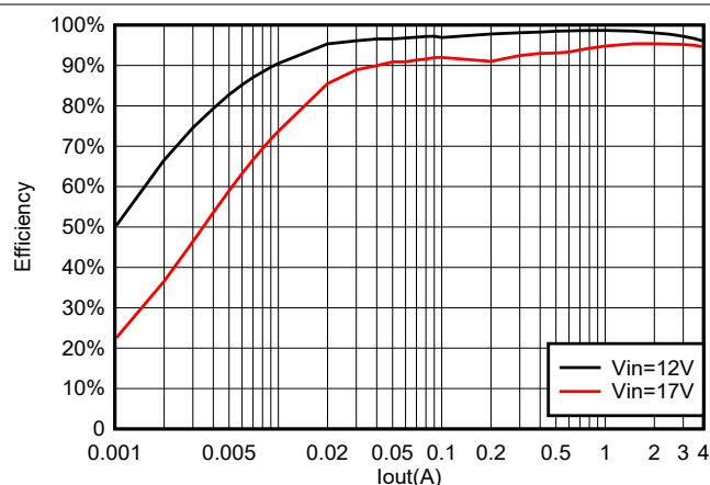
Figure 6-24. TPS564255 Efficiency at 10 V OUT with a 6.8-μH Inductor
