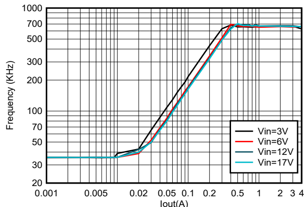
Figure 8-4. TPS564255 Frequency vs Loading
