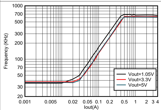
Figure 6-12. TPS564255 Frequency vs Loading, V_{IN} = 12\text{ V}
