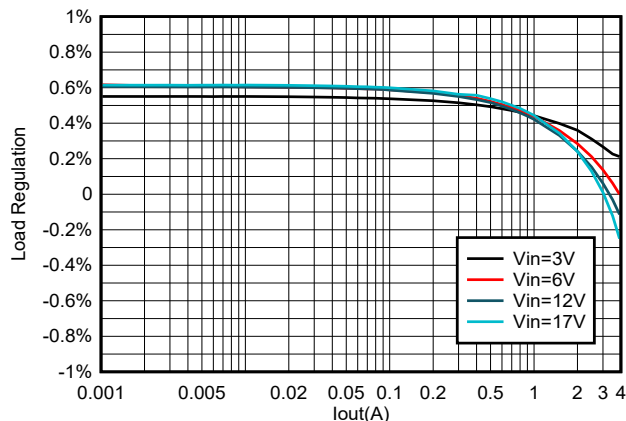
Figure 8-5. TPS564252 Load Regulation vs Loading
