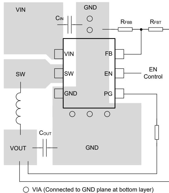
Figure 8-26. Suggested Layout
