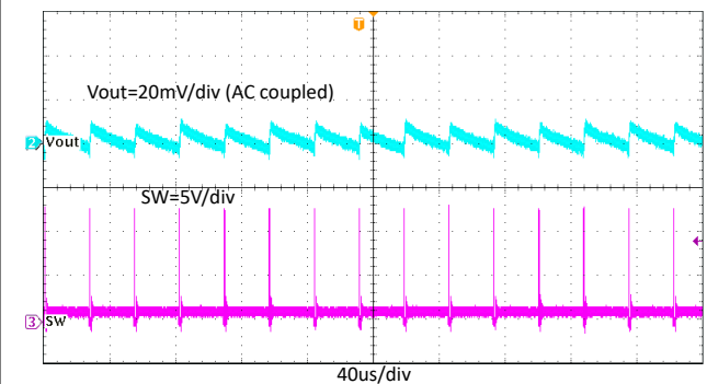
Figure 8-13. TPS564255 Output Voltage Ripple with 0.01-A Loading
