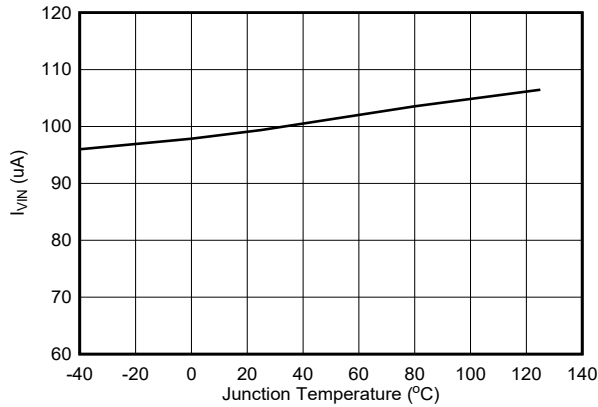
Figure 6-1. TPS564252 Quiescent Current
