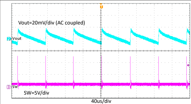
Figure 8-11. TPS564252 Output Voltage Ripple with 0.01-A Loading
