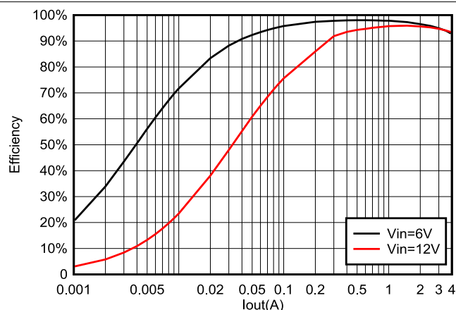
Figure 6-20. TPS564257 Efficiency at 5 V OUT with a 4.7-μH Inductor
