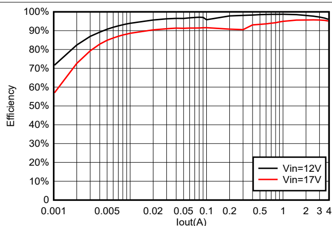
Figure 6-22. TPS564252 Efficiency at 10 V OUT with a 6.8-μH Inductor
