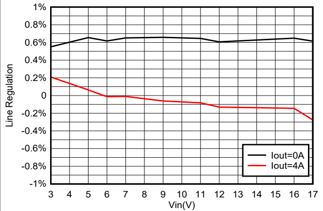
Figure 8-9. TPS564257 Line Regulation vs V_{IN}
