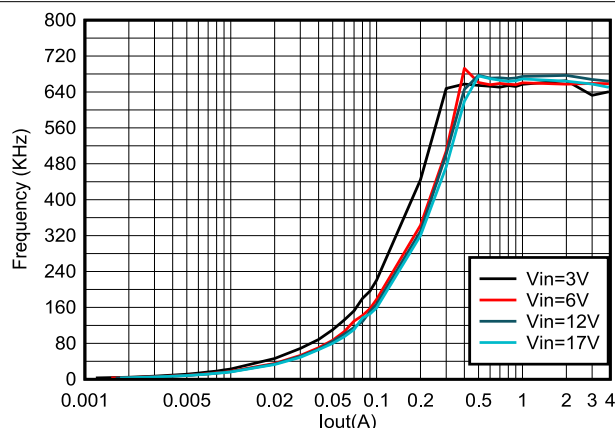
Figure 8-2. TPS564252 Frequency vs Loading
