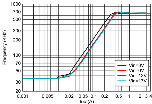
Figure 8-4. TPS564255 Frequency vs Loading
