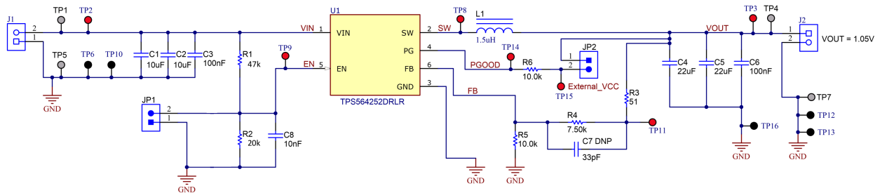
Figure 8-1. Schematic
