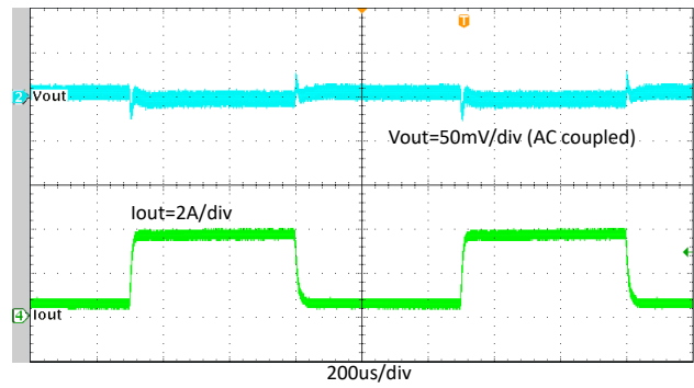
Figure 8-15. TPS564252 Transient Response with 0.4 A to 3.6 A
