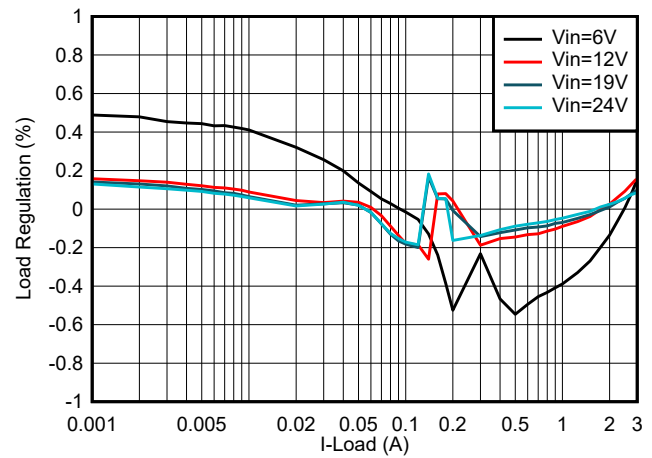
Figure 8-3. Load Regulation
