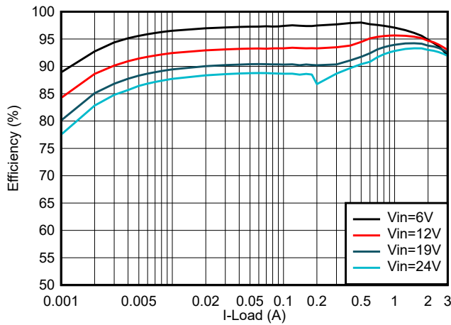
Figure 8-2. Efficiency
