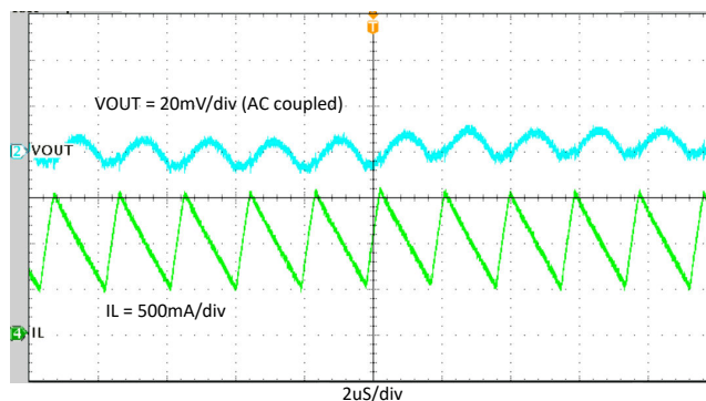
Figure 8-15. Steady State, I_{OUT} = 1 A
