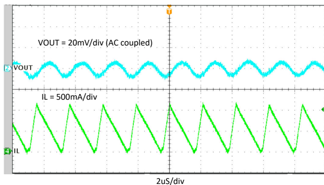
Figure 8-14. Steady State, I_{OUT} = 0.5 A
