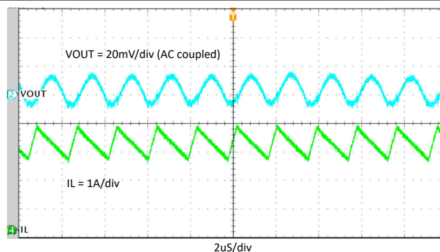
Figure 8-17. Steady State, I_{OUT} = 3 A
