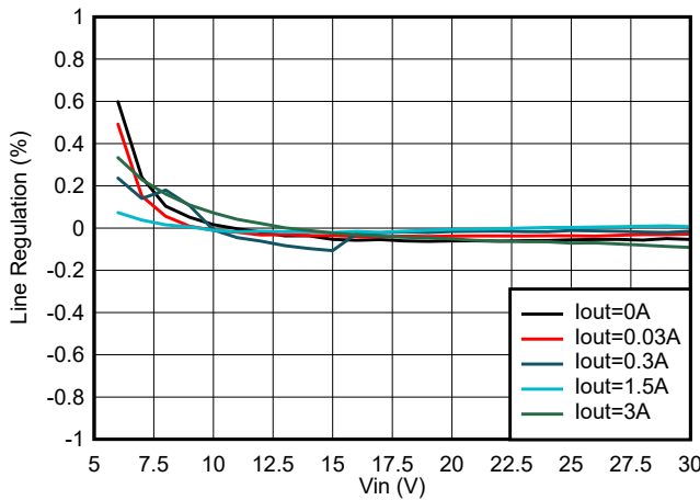
Figure 8-4. Line Regulation
