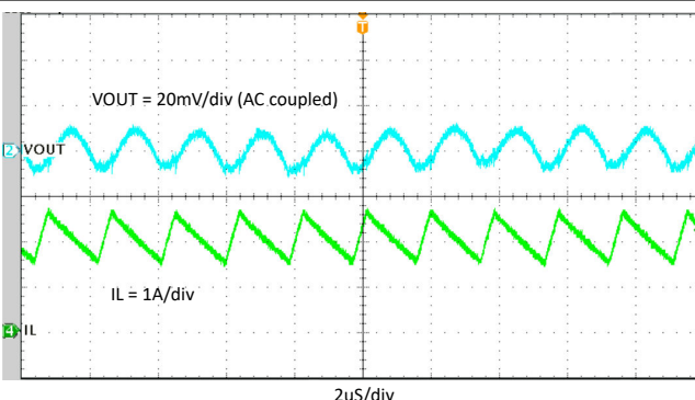
Figure 8-16. Steady State, I_{OUT} = 2 A
