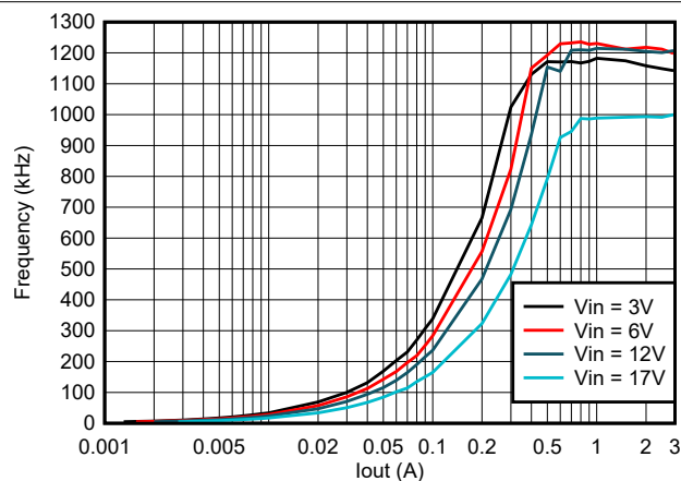
Figure 8-2. TPS563252 Frequency vs Loading
