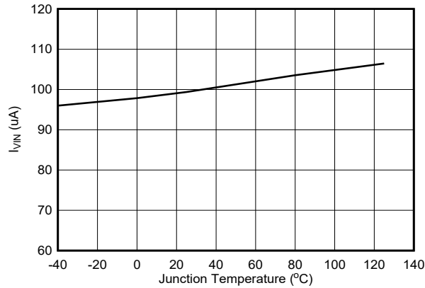
Figure 6-1. TPS563252 Quiescent Current
