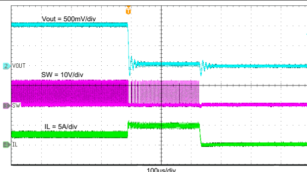
Figure 8-19. TPS563252 Normal Operation to Output Hard Short
