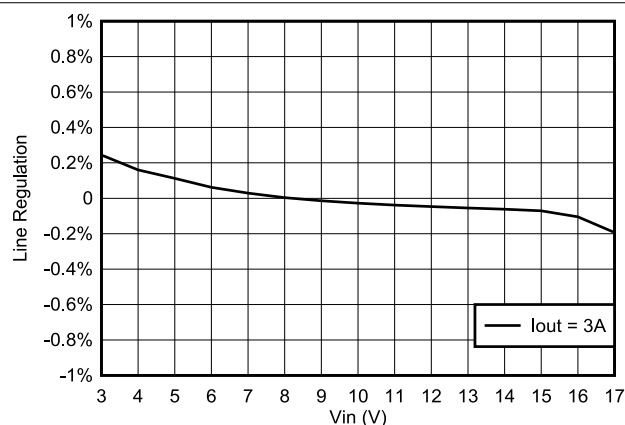
Figure 8-6. TPS563252 Line Regulation vs V_{IN}
