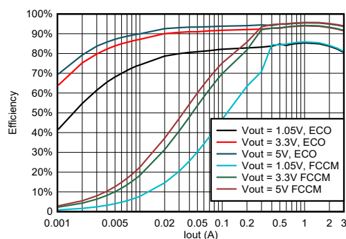
TPS56325x Efficiency at V_{\text{IN}} = 12\text{ V}
