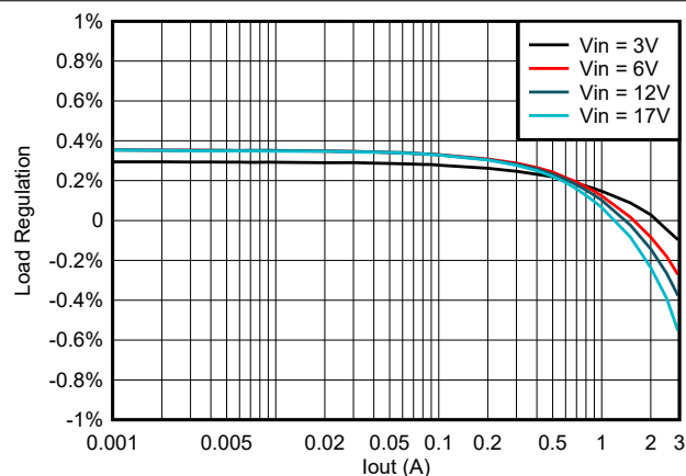
Figure 8-4. TPS563252 Load Regulation vs Loading
