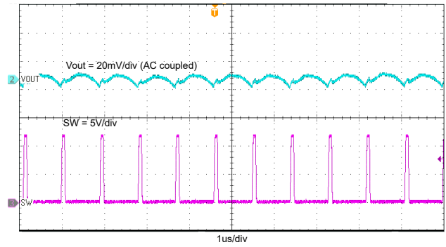
Figure 8-9. TPS563257 Output Voltage Ripple with 0.01-A Loading
