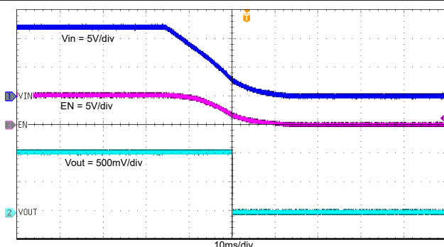
Figure 8-18. Shutdown with V_{IN} Falling, I_{OUT} = 3\text{ A}
