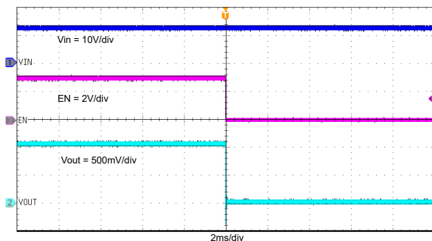
Figure 8-16. Shutdown Through EN, I_{OUT} = 3\text{ A}
