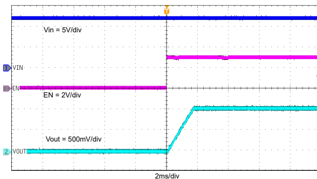
Figure 8-15. Start-Up Through EN, I_{OUT} = 3\text{ A}
