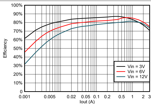
Figure 6-11. TPS563252 Efficiency at 0.6 V_{OUT} with a 0.68- \mu\text{H} Inductor
