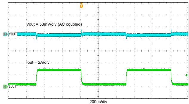
Figure 8-13. TPS563257 Transient Response with 0.3 A to 2.7 A
