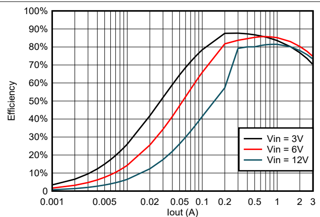
Figure 6-12. TPS563257 Efficiency at 0.6 V_{OUT} with a 0.68- \mu\text{H} Inductor
