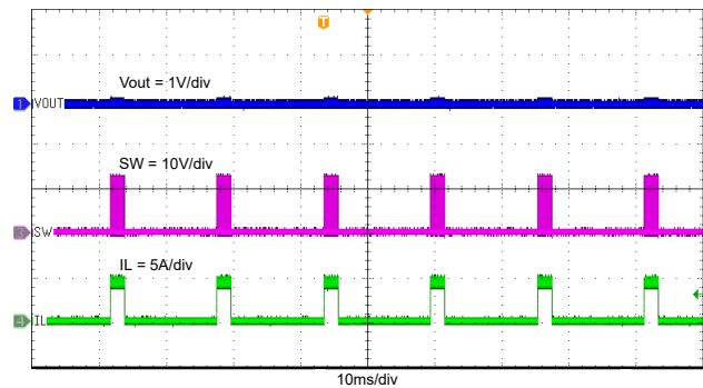
Figure 8-21. Output Hard Short Hiccup
