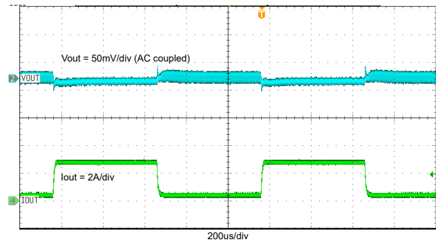
Figure 8-11. TPS563252 Transient Response with 0.3 A to 2.7 A
