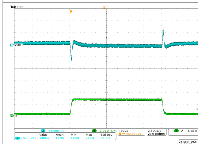
Figure 8-10. Transient Response 0.3 to 2.7 A with Slew Rate of 2.5 A/μs
