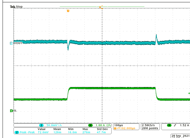
Figure 8-12. Transient Response 1 to 2 A with Slew Rate of 2.5 A/μs
