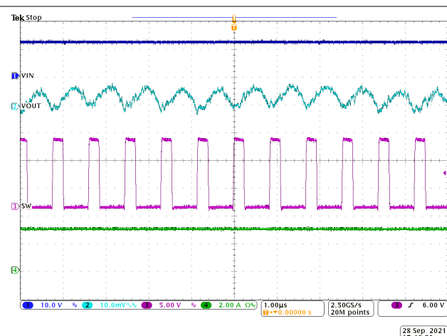
Figure 8-9. Steady State Waveforms, I_{OUT} = 3 A
