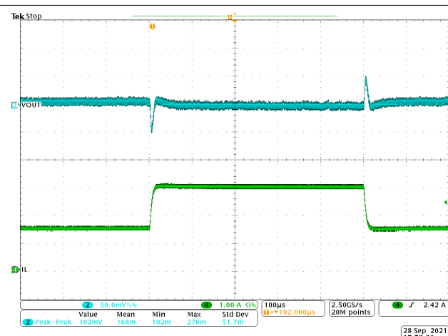
Figure 8-13. Transient Response 1.5 to 3 A with Slew Rate of 2.5 A/μs
