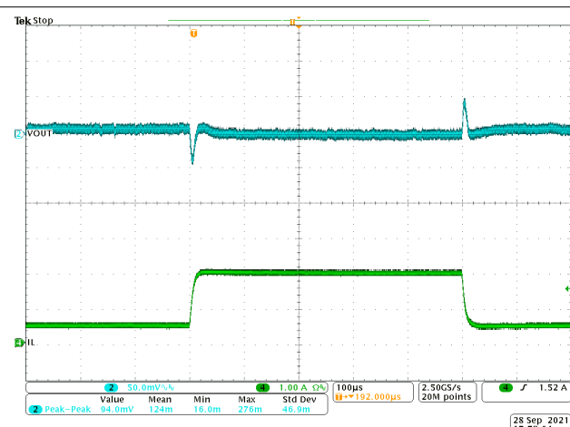
Figure 8-11. Transient Response 0.5 to 2 A with Slew Rate of 2.5 A/μs
