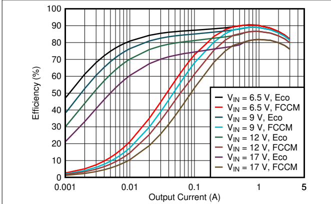
Figure 6-13. V_{OUT} = 1.05\text{-V} Efficiency, L = 1.5\ \mu\text{H}
