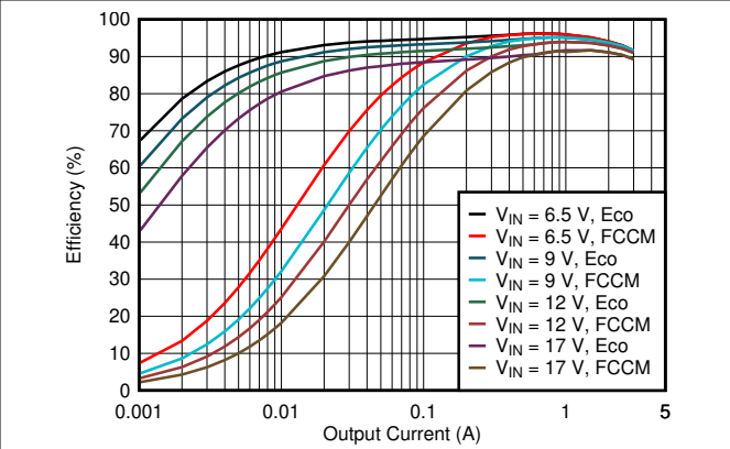
Figure 6-14. V_{OUT} = 3.3\text{-V} Efficiency, L = 3.3\ \mu\text{H}
