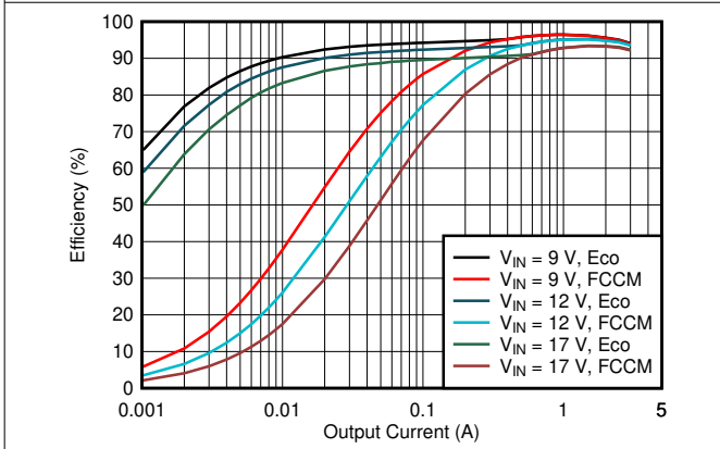
Figure 6-15. V_{OUT} = 5\text{-V} Efficiency, L = 4.7\ \mu\text{H}
