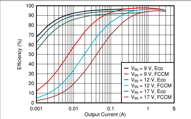
Figure 6-16. V_{OUT} = 7\text{-V} Efficiency, L = 4.7\ \mu\text{H}
