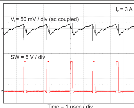
Figure 8-22. Tps563200 Input Voltage Ripple
