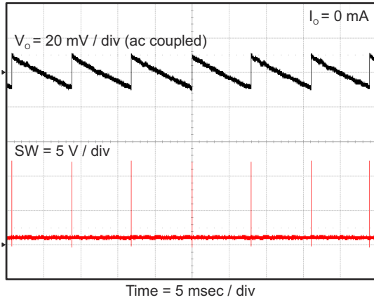
Figure 8-23. Tps563200 Output Voltage Ripple
