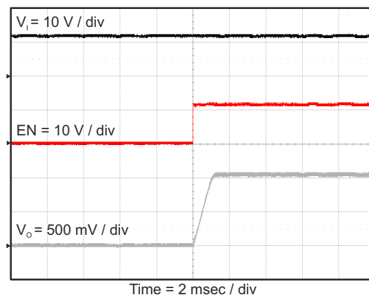
Figure 8-13. TPS562200 Start Up Relative to En
