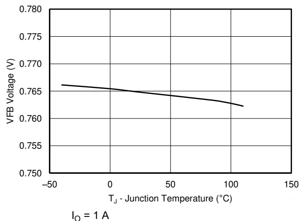
Figure 6-3. Vfb Voltage vs Junction Temperature
