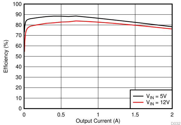
Figure 8-2. Tps562200 Efficiency
