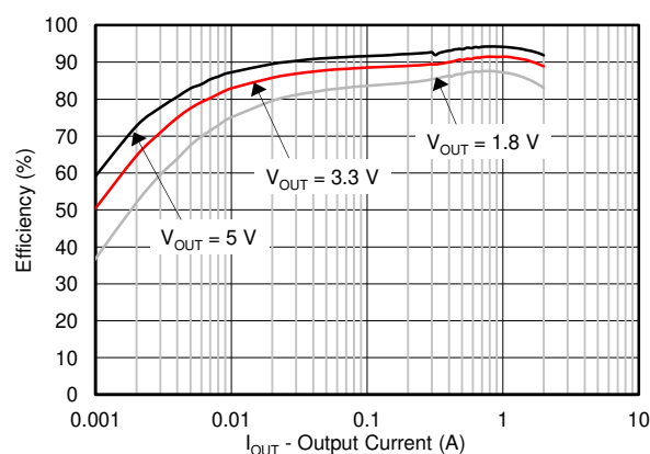
Tps562200 Efficiency
