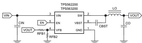
Simplified Schematic
