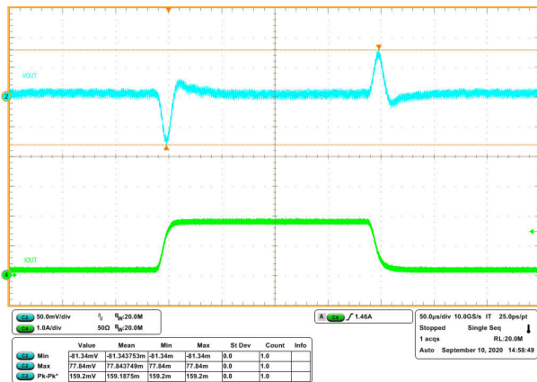
Figure 8-14. Transient Response 0.2 to 1.8 A with Slew Rate of 0.25 A/ \mu s (FCCM)
