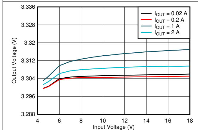
Figure 8-4. Line Regulation
