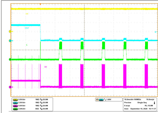
Figure 8-20. Output Short Protection
