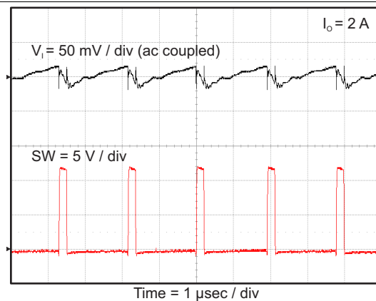
Figure 23. TPS562210A Input Voltage Ripple
