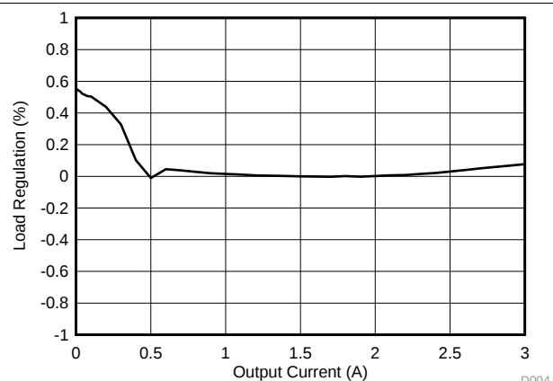
Figure 36. TPS563210A Load Regulation, V_I = 12 V
