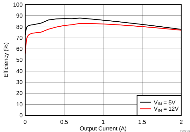
Figure 18. TPS562210A Efficiency
