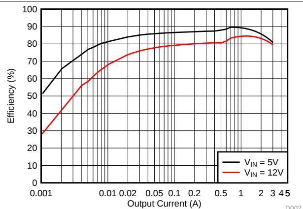
Figure 34. TPS563210A Light Load Efficiency
