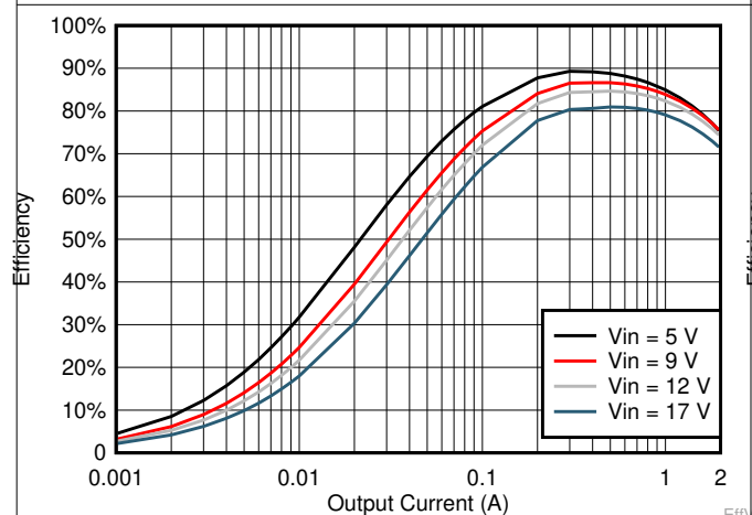
Figure 6-9. V_{OUT} = 0.95\text{ V} Efficiency, L = 2.2\mu\text{H}
