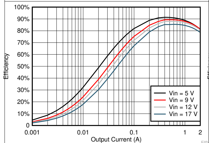
Figure 6-11. V_{OUT} = 1.5\text{ V} Efficiency, L = 2.2\mu\text{H}
