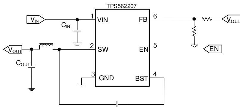
Simplified Schematic
