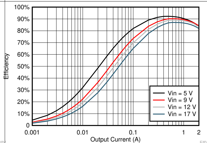
Figure 6-12. V_{OUT} = 1.8\text{ V} Efficiency, L = 2.2\mu\text{H}
