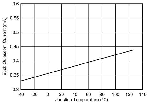
Figure 7-1. Supply Current vs Junction Temperature
