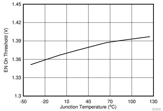
Figure 7-4. EN On Threshold Voltage vs Junction Temperature
