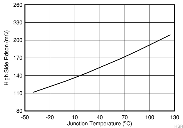
Figure 7-5. High-Side R_{ds-On} vs Junction Temperature
