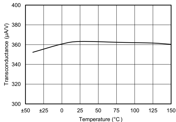
Figure 6-1. Error Amplifier Transconductance vs Temperature
