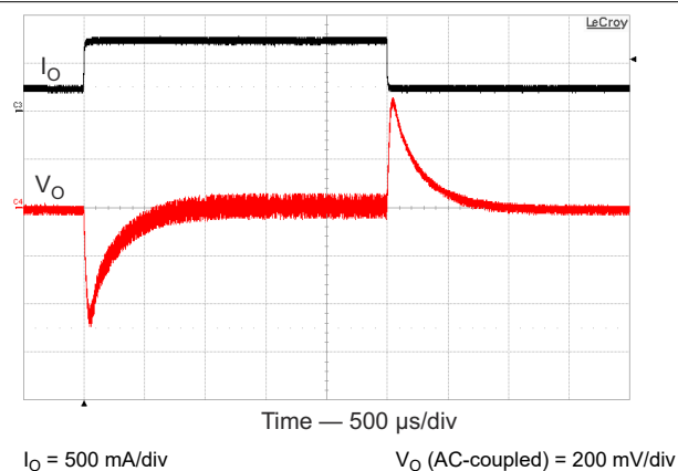
Figure 8-13. Load Transient Response
