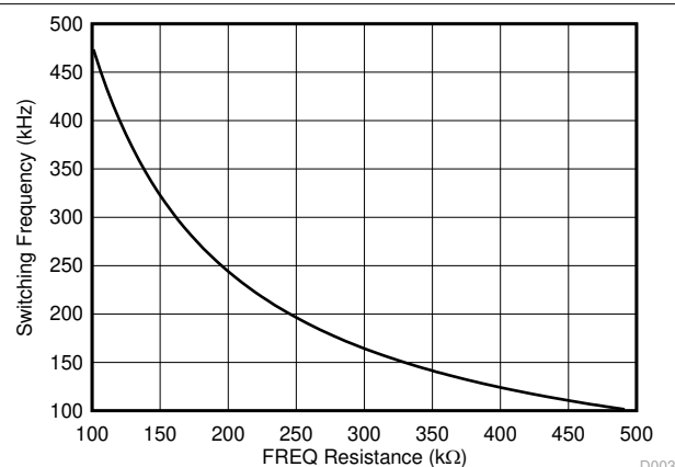
Figure 6-5. Frequency vs FREQ Resistance Low Frequency Range
