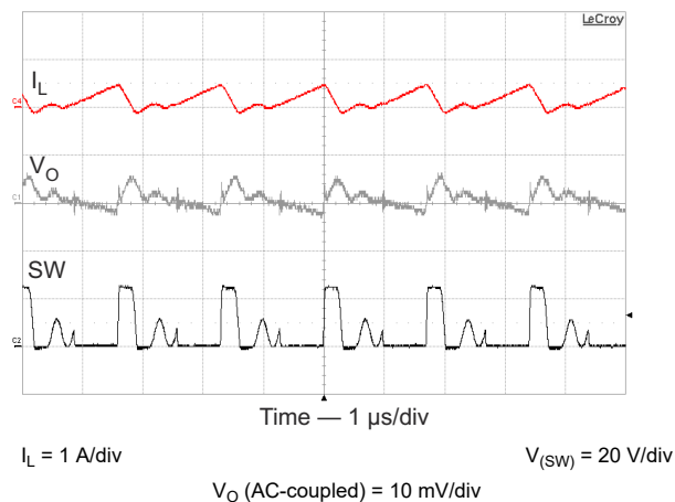
Figure 8-6. DCM PWM Operation
