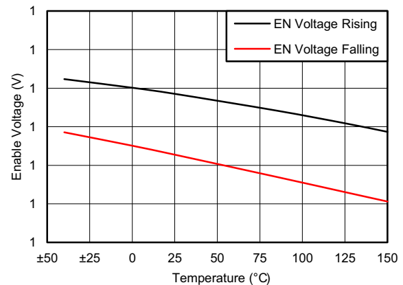
Figure 6-12. Enable Voltage vs Temperature
