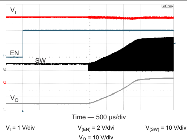
Figure 8-8. Start-Up
