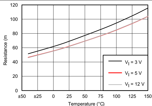
Figure 6-4. Static Drain Source On-State Resistance ( r_{\text{DS(on)}} ) vs Temperature
