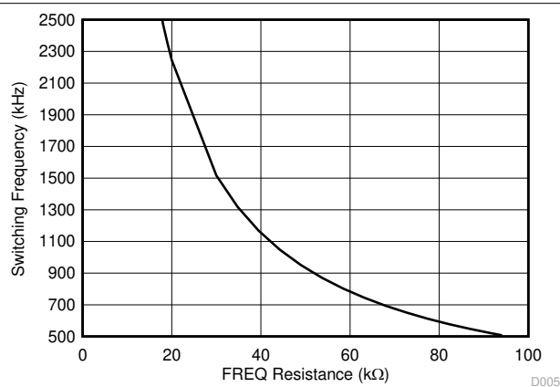
Figure 6-6. Frequency vs FREQ Resistance High Frequency Range
