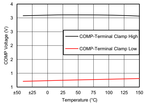
Figure 6-10. COMP Clamp Voltage vs Temperature
