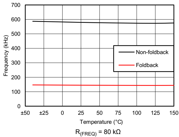
Figure 6-9. Non-Foldback Frequency vs Foldback Frequency
