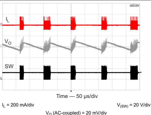
Figure 8-7. Pulse Skipping
