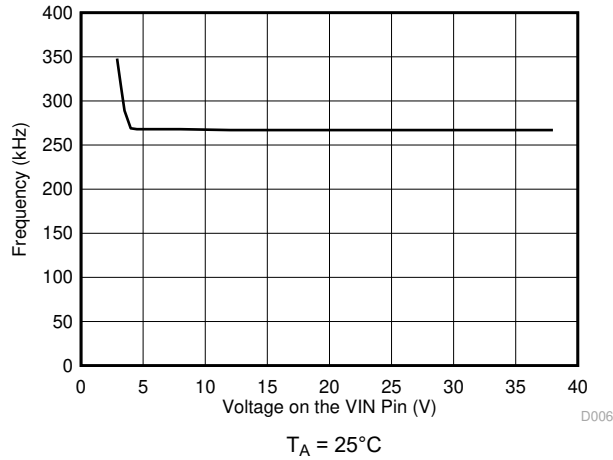
Figure 6-7. Minimum Switching Frequency for Quick Recovery from Frequency Foldback
