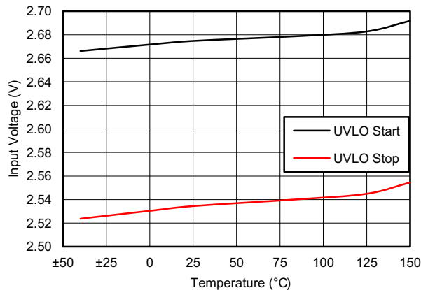
Figure 6-11. Input Voltage UVLO vs Temperature
