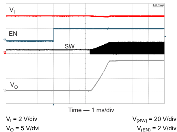
Figure 8-15. Output Voltage Soft Start
