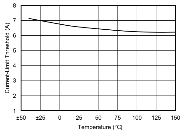
Figure 6-2. Switch Current Limit vs Temperature
