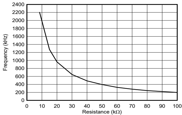
Figure 6-11. Switching Frequency vs Setting Resistance
