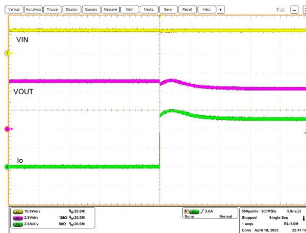
Figure 8-12. Output Current Limit Waveforms in V_{IN} = 12\text{ V} , V_{OUT} = 5\text{ V} , R_{LOAD} = 0.8\text{ }\Omega , R_{SNS} = 10\text{ m}\Omega , FPWM
